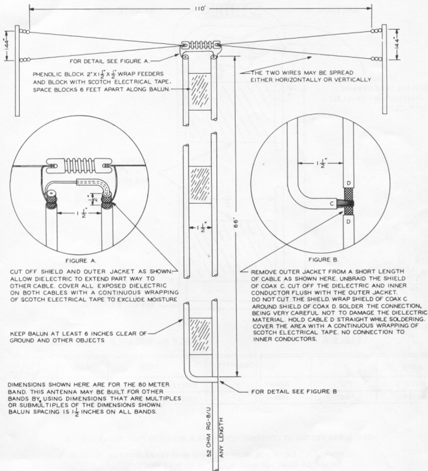
Figure 5. Broadband Antenna with Quarter Wave Unbalanced to Balanced Transformer (Balun) Feed System
