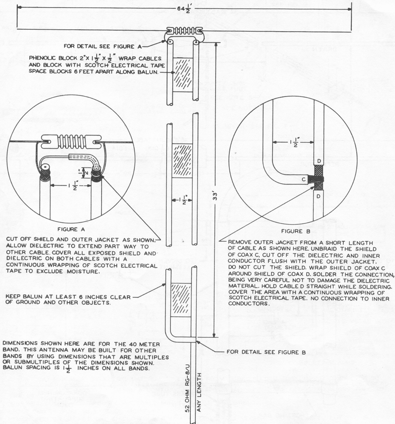
Figure 4. Half Wave Antenna with Quarter Wave Unbalanced to Balanced Transformer (Balun) Feed System
